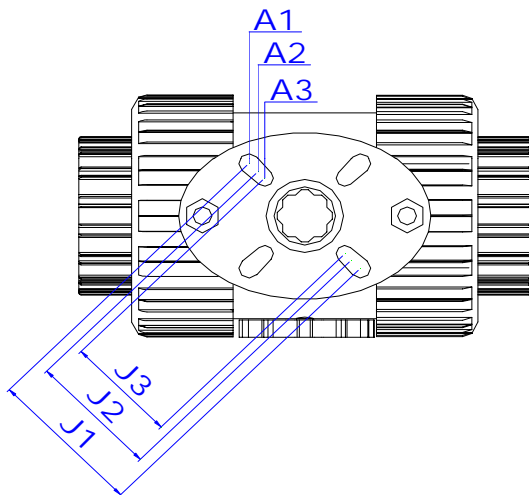
DN15, DN20 AND DN25 VALVE
