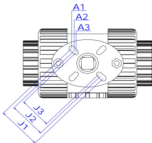
DN15, DN20 AND DN25 VALVE
